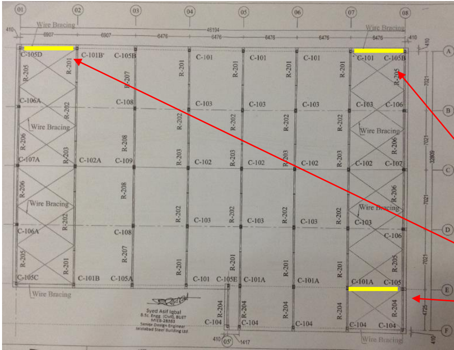
Lack of vertical bracing
